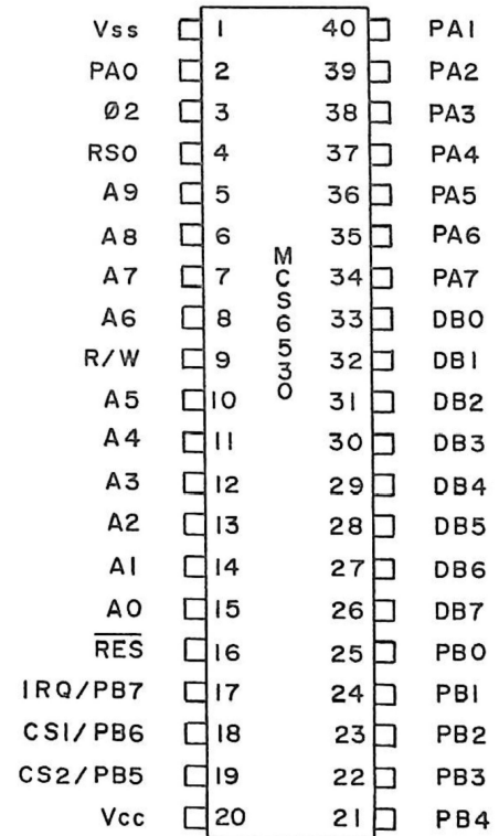
PIN DESIGNATION
